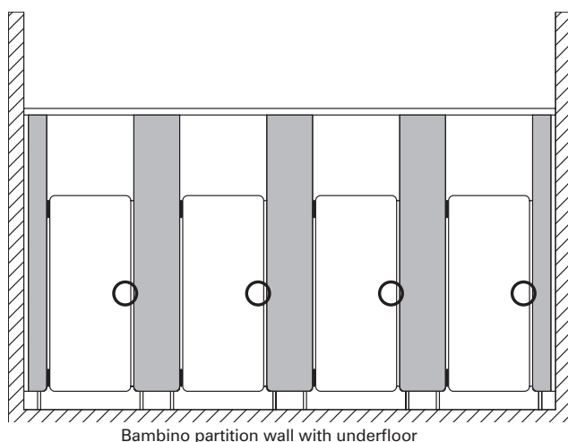
Bambino partition wall with underfloor
